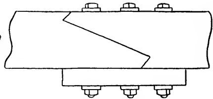
SCARF JOINT
